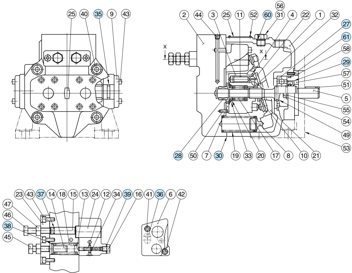
Section X-X
